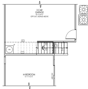
Partial Optional Main Floor Plan
