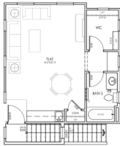
Optional (flat) Upper Floor Plan
